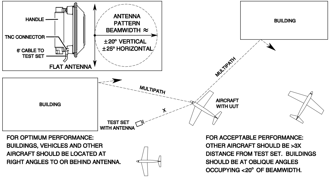
Suggested Layout to Reduce Multipath Errors Figure 26
