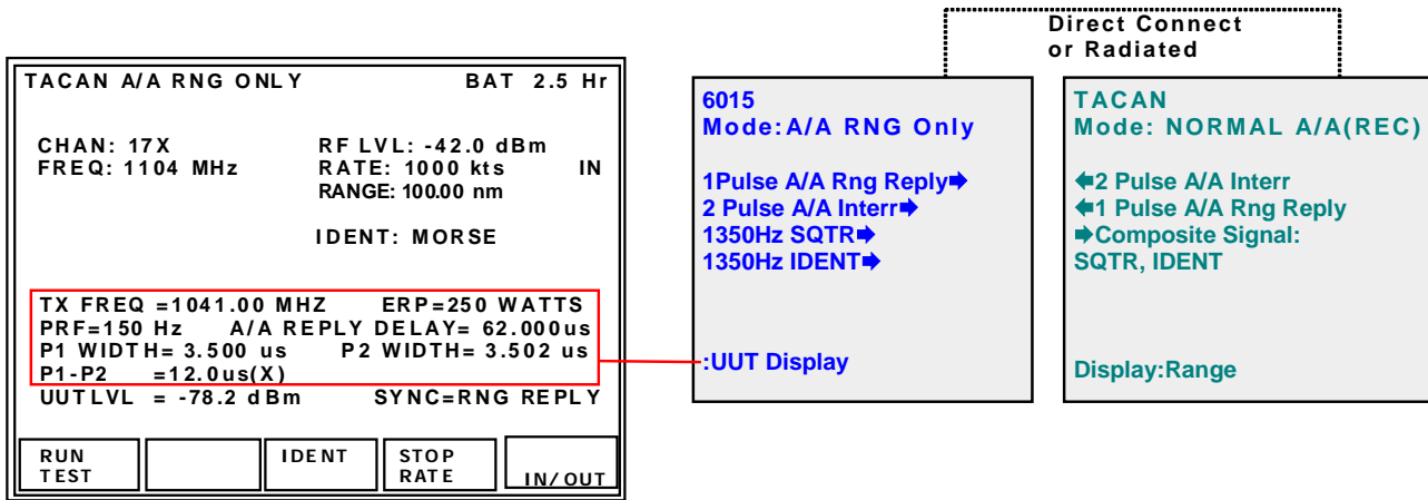
TACAN A/A Range Only Mode Screen Figure 20
