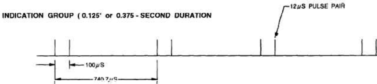
TACAN Pulse Signals Figure 13
